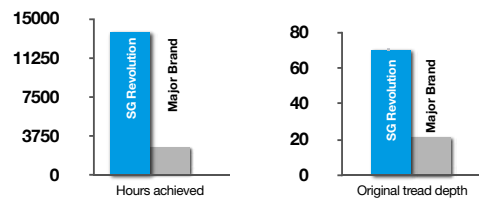
1300 x 24 SG revolution tyres versus 15.5/80R25 Major Brand Radial on JCB Telehandler in Waste Transfer PGC Demolition
