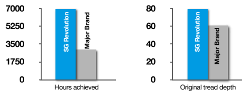
1300 x 24 SG revolution tyres versus 1200x24 Major Brand Radial L5 on JCB Telehandler in Waste Transfer H Martin
