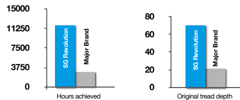
1300 x 24 SG revolution tyres versus 15.5/80R24 Major Brand Radial on JCB Telehandler in Demolition Amgen Cymru
